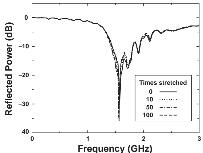
Figure 4. Frequency response of the reflected power from the antenna after repeated stretching up to a strain of 50 %. Plots show the reflected power after the antenna had been stretched 10, 50, and 100 times. The results demonstrated that the resonance frequency and the radiation efficiency of the antenna were almost unchanged (within 1 %) after the antenna had been stretched 100 times.
