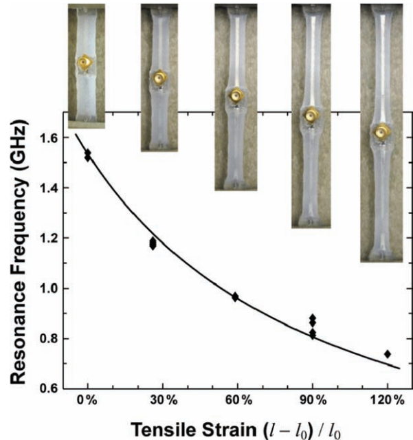
Figure 3. The resonance frequency (GHz) of the antenna as a function of the tensile strain. The resonance frequency of the antenna decreased from 1.53 GHz to 0.738 GHz as the antenna was stretched from l_0 to l = 2.20 l_0 . After releasing the strain, the resonant frequency returned from 0.738 GHz to 1.53 GHz: the tuning is thus reversible. Measurement under each value of strain was repeated five times; and the data points are shown as individual diamonds ( \blacklozenge ) in the plot. The fitted curve was calculated using Equation (1) with \epsilon_{\text{eff}} = 2.1 .
