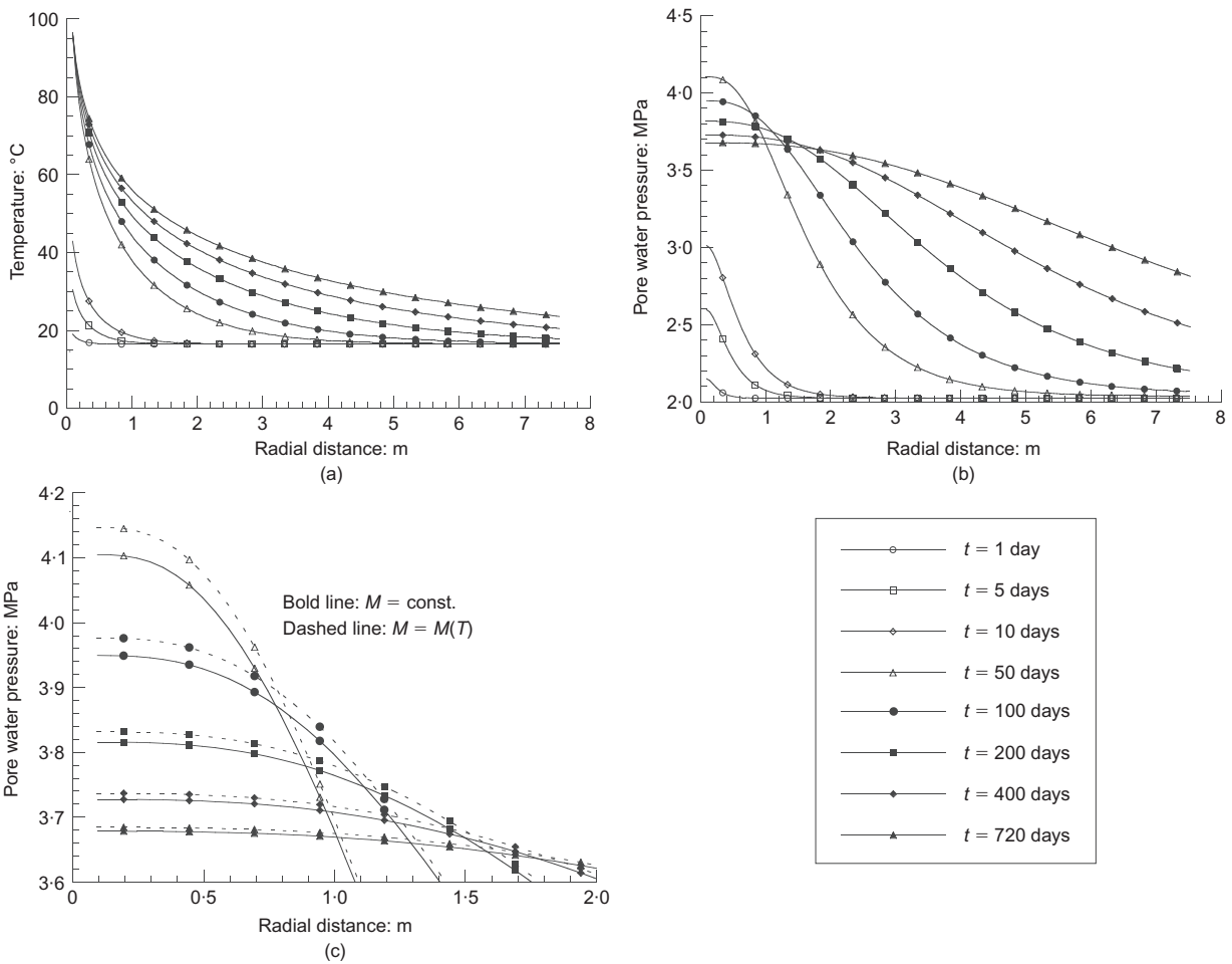
Fig. 2. Evolution of: (a) temperature (identical for both M = \text{const.} and M(\Delta T) ); (b) pore water pressure distribution around heat source (negligible dependence on M(\Delta T) over most of field); (c) pore water pressure in closest vicinity of heat source, showing limited dependence on M
