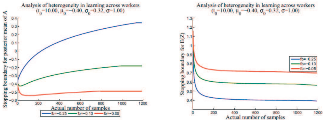
Figure 2: Stopping boundaries for different learning rates
