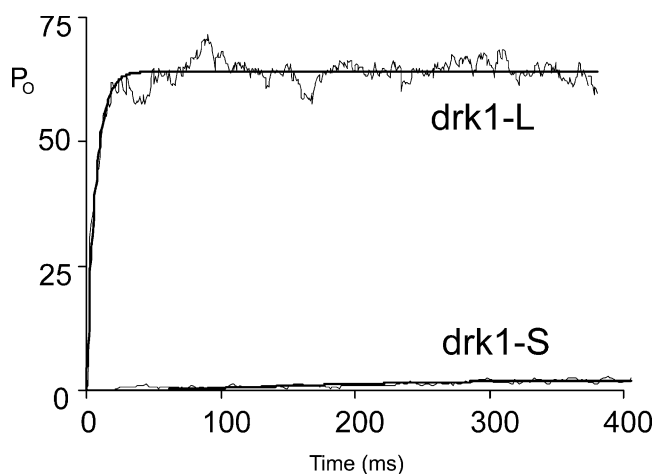
Figure 4. Ensemble averages for drk1-L and drk1-S. Probability of being open following a step depolarization to 0 mV in patches containing N channels ( NP_O ), where N = 1 for drk1-L, and N \geq 1 for drk1-S (see Fig. 3). NP_O was obtained from ensemble averages after records were idealized by the TRANSIT algorithm (VanDongen, 1996, 2004a). Ensemble averages (thin line) were fit with the following model modified after Hodgkin and Huxley (1952): P_O(t) = n_{inf} * [1 - \exp(-t/\tau_n)]^Q . n_{inf} is the steady-state open probability, \tau_n is the activation time constant, and (Q) is the exponent. The thick line illustrates the optimal fit. Optimized parameters were as follows: for drk1-L: \tau_n = 6.29 ms, n_{inf} = 0.641 , Q = 1.05 , and for drk1-S: \tau_n = 112.0 ms, n_{inf} = 0.024 , Q = 1.00 .
