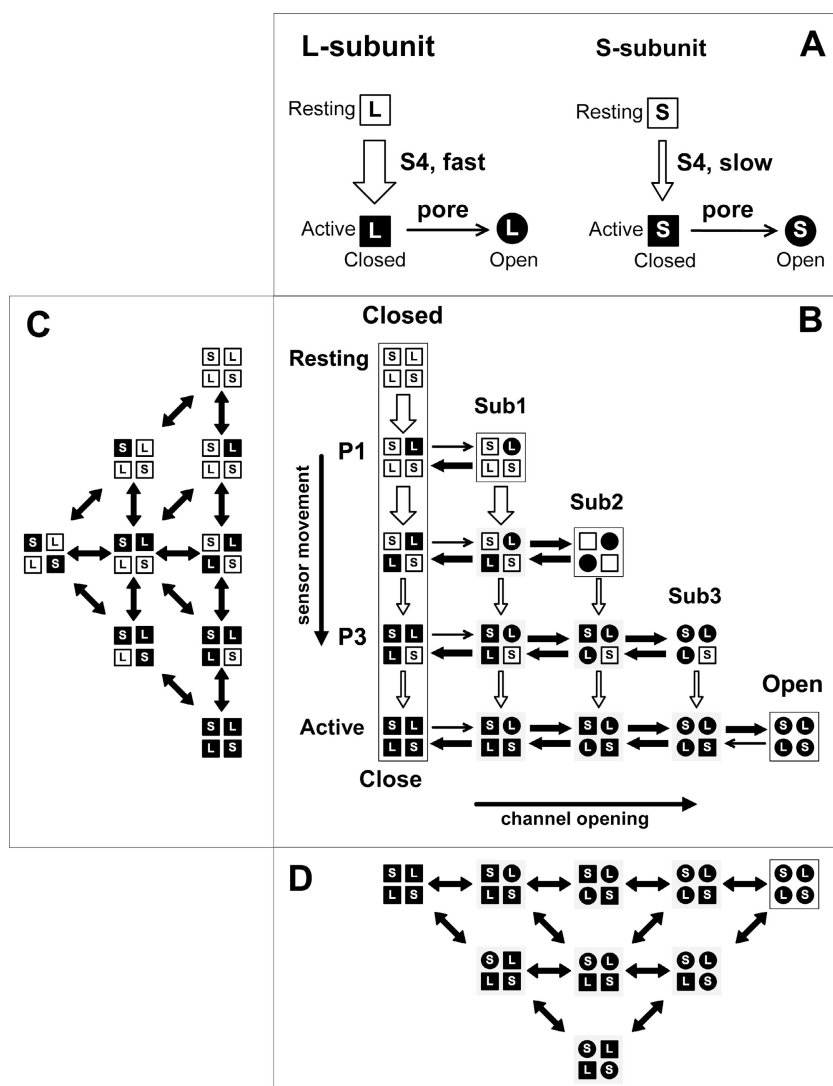
Figure 5. Subunit-subconductance model for voltage-gated K channels. The open \leftrightarrow close behavior illustrated in Fig. 1 G reflects the intrinsic kinetic properties of the gate, as described by the model in Fig. 1 A. In voltage-gated channels, this intrinsic gating behavior is allosterically controlled by membrane potential. A subunit-based kinetic scheme for K channels assembled from two S and two L subunits is constructed as follows. (A) The drk1-S and drk1-L subunits are modeled separately, since they differ in their voltage dependence. As before, each subunit is described by a linear three-state model that directly couples voltage sensor movement to channel opening. Closed states are represented by squares, open states by circles. Open squares indicate a resting voltage sensor; filled squares/circles imply the sensor has moved. The direction of the arrows specifies the position of the equilibrium and the width of the arrow the relative magnitude of the rate constants. The direction and width of the arrows are reflective of a membrane potential of 0 mV. Open arrows are voltage dependent (and involve sensor movements), closed arrows are voltage independent (indicating open–close gating transitions). (B–D) Combining two S and two L subunits in an S-L-S-L configuration results in a complex three-dimensional 36-state model. However, at intermediate membrane potentials, S-L channels will preferentially visit a subset of states, because the L subunits are likely to activate before the S subunits. The preferred itinerary is shown by the 15-state triangular model in B, while C and D illustrate all possible activation and opening transitions, respectively. The 15-state model contains three functionally homomeric states, at the corners of the triangle. Voltage sensor movements are represented by vertical transitions, open–close transitions by horizontal arrows. Rows labeled P1–P3
