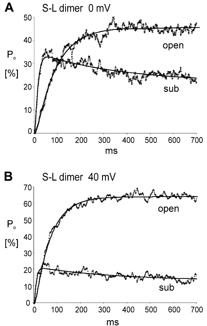
Figure 8. Activation kinetics of sublevels and the fully open state in the S-L dimer. (A and B) Probabilities of being in the fully open state or a subconductance level as a function of time after the step depolarization at both 0 and +40 mV were estimated by ensemble averages following idealization and interpretation by TRANSIT (VanDongen, 1996). The P_o curves were fitted with a sum of three exponentials plus a constant ( a_0 ), shown by the solid line. P_o(t) = a_0 + a_1 \exp(-t/\tau_1) + a_2 \exp(-t/\tau_2) + a_3 \exp(-t/\tau_3) . The optimal values in the format a_0, \tau_1 (a_1), \tau_2 (a_2), \tau_3 (a_3) were as follows: for sublevels at 0 mV, 21.8, 367 (13.3), 8.48 (-3813), 8.40 (3777); for the open state at 0 mV, 45, 11.3 (7.4), 81.4 (16.7), 84.4 (-69.8); for sublevels at +40 mV, 13.1, 365 (8.6), 5.40 (-3812), 5.36 (3790); for the open state at +40 mV, 63.8, 9.3 (15), 58.7 (1.0), 60.7 (-79.8). Time constants ( \tau_1 - \tau_3 ) are in ms, their amplitudes ( a_1 - a_3 ) in percentages.
