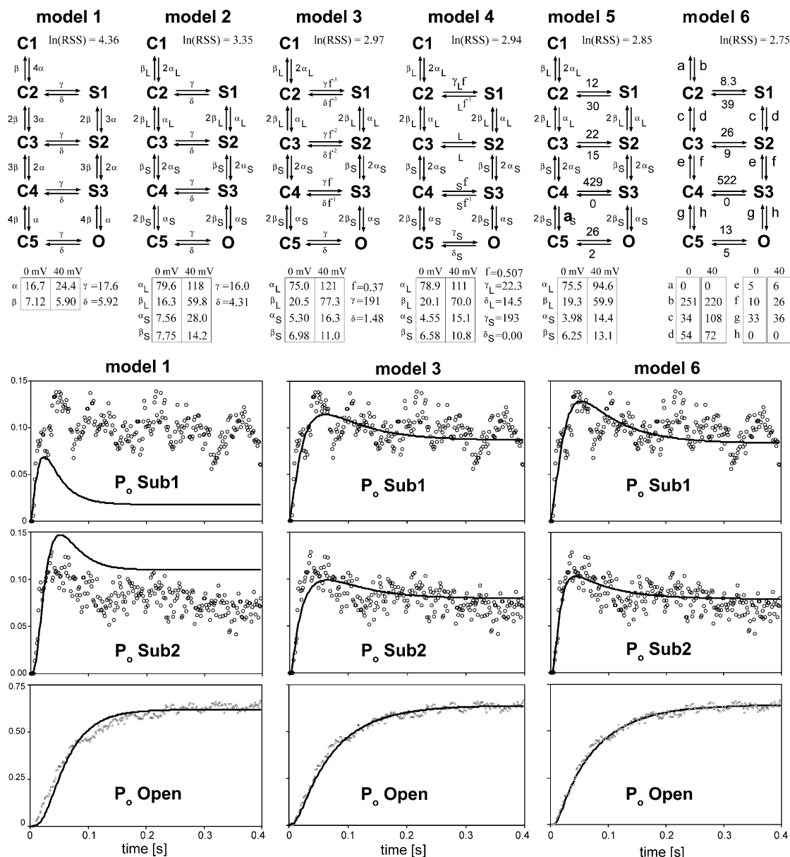
Figure 12. Subunit-subconductance models. To investigate whether the subunit-subconductance model can accurately describe the single channel behavior of the S-L dimer, Markov models were generated that represent specific instances of the general model shown in Fig. 5 B. The six extremely short-lived sublevels, which have a gray background in Fig. 5 B, were omitted from the Markov models, since the majority of visits to these levels will go undetected due to the low pass filtering. This results in nine resolvable states: five closed states (C1–C5), three sublevels (S1–S3), and the open state (O). Six variations were used (models 1–6) for which the number of free (optimized) parameters increases with the model, by reducing the number of constraints. Each Markov scheme defines a set of nine differential equations that were integrated to generate models of P_o(t) , FL(t) , and COP(t) for Sub1, Sub2, and Open, at 0 and +40 mV (a total of 18 curves). Activation rate constants (vertical transitions) depend on membrane potential; rate constants describing channel opening (horizontal transitions) are voltage independent. For the P_o(t) and FL(t) curves, it was assumed that all channels are in C1 at t = 0 . The initial conditions for the COP(t) curves are not known and were therefore estimated. There are nine Markov states for three COP curves (Sub1, Sub2, Open) at two membrane potentials, resulting in 54 initial conditions to be estimated. In addition, rate constants and allosteric factors were estimated for each model by minimizing the sum of squared residuals (RSS) between the data and the model using the Solver in Microsoft Excel. Optimized values are provided for each model. The natural log of the residual sum of squares (RSS) is shown for each model as a relative measure of goodness-of-fit. Model 1 is the most severely constrained model and it makes two assumptions: (1) that there are four identical and independent voltage sensors, and (2) that opening transitions do not depend on the number of activated subunits. These constraints result in a model with only six free rate constants. The model provided a very poor description of the data, as illustrated by the P_o(t) curve fits below. Model 2 takes into account that the S-L dimer contains subunits with distinct voltage sensors. Activation is described by two fast L sensors and two slower S sensors. Voltage sensors still move independently, and opening transitions do not depend on the number of activated subunits. This model has 10 free rate constants. Model 3 improves upon model 2 by
