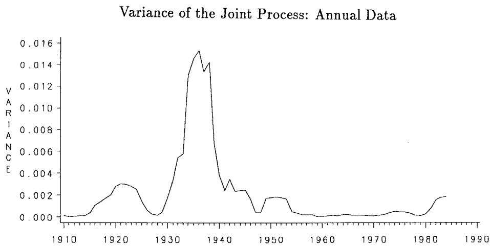
Fig. 12. Moving Window Estimates of the Joint Processes Quarterly and Annual Data. The top panel plots the quarterly data. Plotting symbols 1 to 4 represent the maturity of the interest rate in quarters. The window length is three years. In the bottom panel, the annual data is plotted. The window length is five years. In all the calculations, it is assumed that \alpha = 1 and \delta = 1 .
