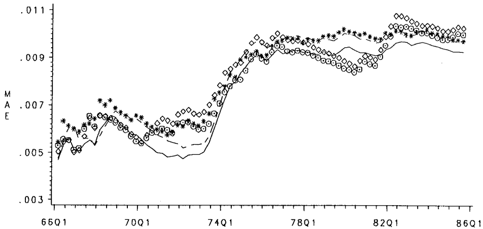
Fig. 17. Root Mean Squared and Mean Absolute Errors of the Three Quarter Ahead Inflation Forecasting Models. The symbols are: Random Walk (Star), Time Series (Line), Time Series Window (Dash), Treasury Bill-Average (Circle) and Treasury Bill-Spot (Diamond).
