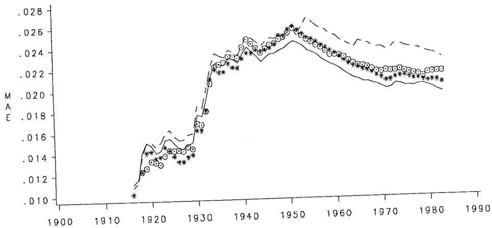
Fig. 7. Root Mean Squared and Mean Absolute Errors of the Inflation Forecasting Models: Annual Data. The symbols are: Random Walk (Star), Time Series (Line), Time Series Window (Dash), Treasury Bill-Average (Circle) and Treasury Bill-Spot (Diamond).
