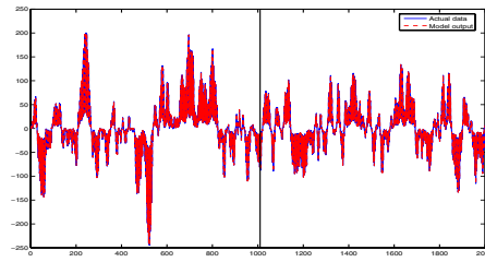
Fig. 10. Example 2: True output y and the output of the identified model \hat{y} . Data to the left of the vertical line were used for identification and the right of the vertical line is prediction using the identified model.
