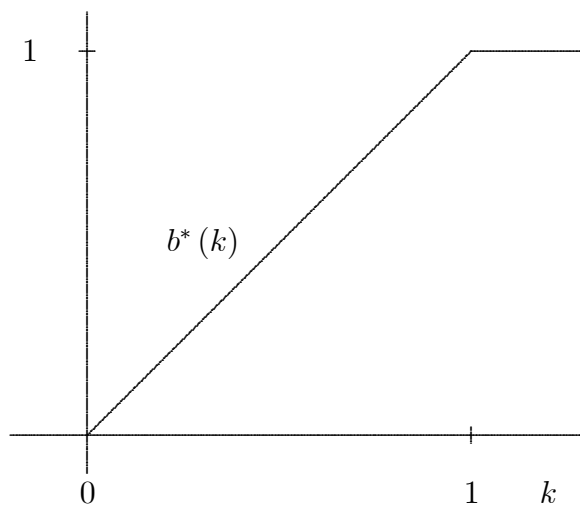
Figure 5.1: Function b^*(k)
