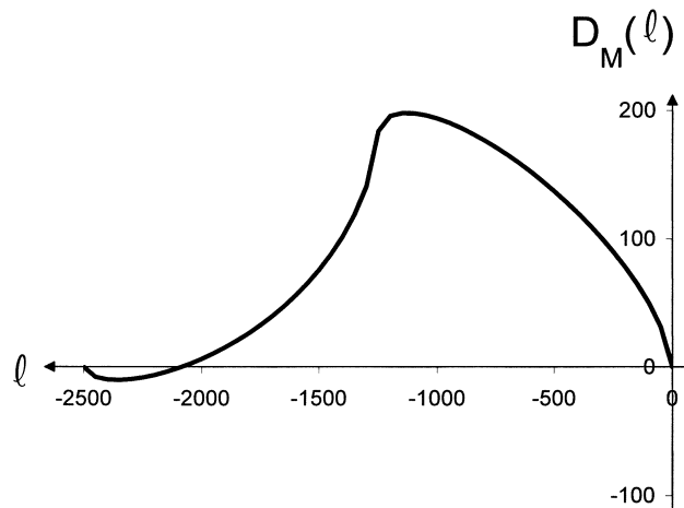
Figure 3.5 D_M(\ell) for \alpha = 0.7 and k = 2.25
