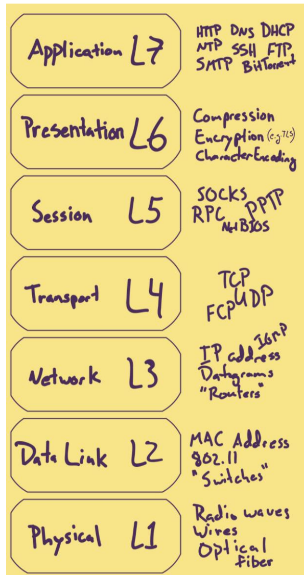
Illustration 1: OSI model layer names and examples
