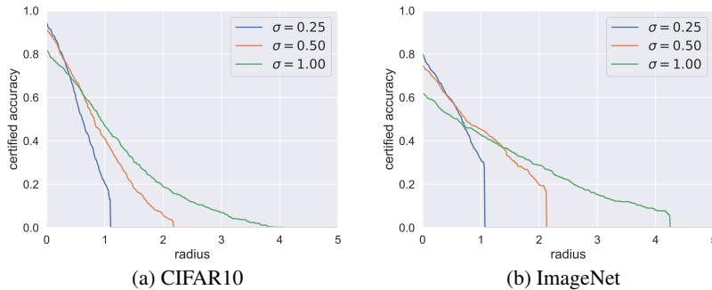
Figure 3: Impact of \sigma on the certified top-3 accuracy.
