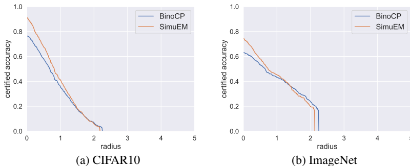
Figure 4: BinoCP vs. SimuEM, where k = 3 .
