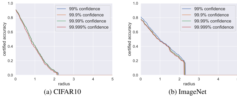
Figure 2: Impact of the confidence level 1 - \alpha on the certified top-3 accuracy.
